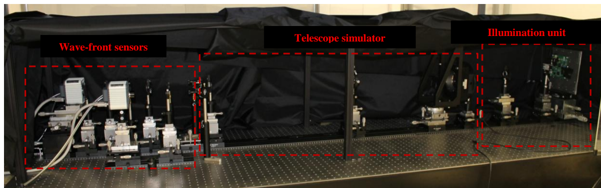
Figure 4 Photograph of the RASCASSE breadboard at LAM RASCASSE breadboard is dedicated for wave-front sensor characterization. This smart set-up is fully representative of the space telescope.
